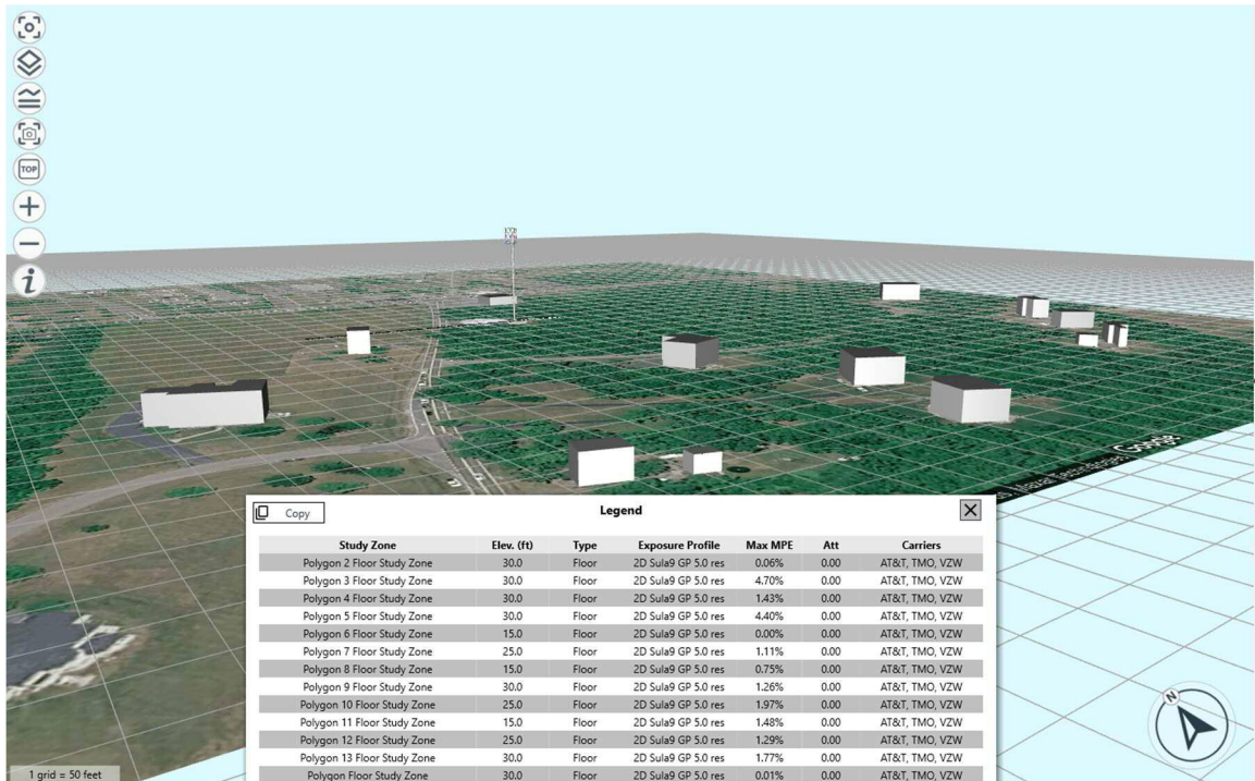
Figure 2 – calculated cumulative exposure level on nearby rooftops surrounding the proposed telecommunications facility expressed in percentage of the applicable FCC standard
