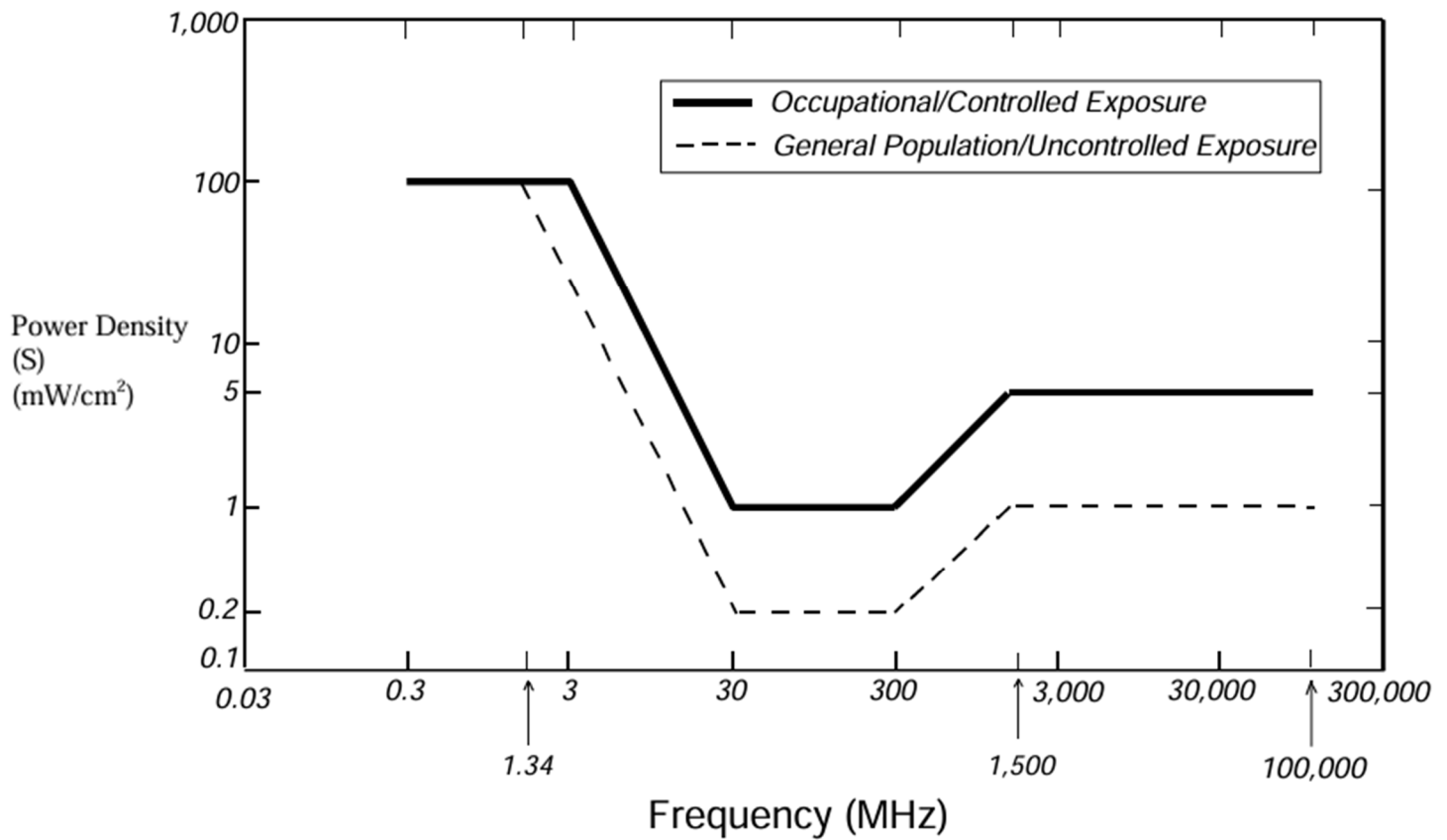
Figure 3 – FCC Limits for Maximum Permissible Exposure (MPE) 1
