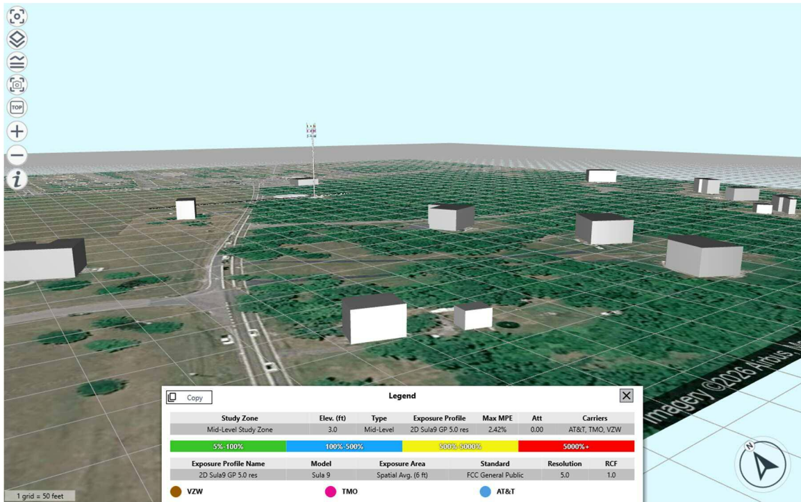
Figure 1 – calculated ground level cumulative exposure level surrounding the proposed telecommunications facility expressed in percentage of the applicable FCC standard
